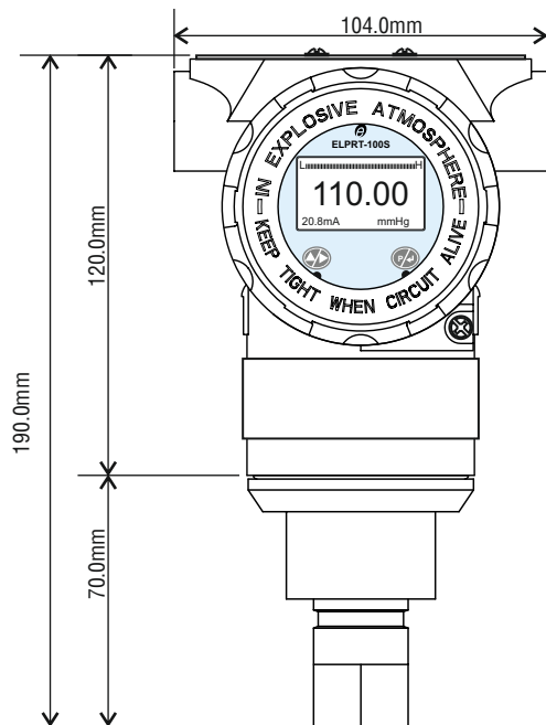
Fig.1 Front View
