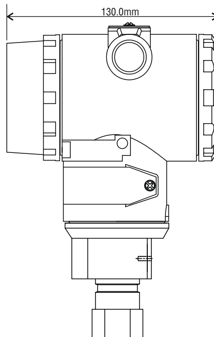
Fig.2 Side View
